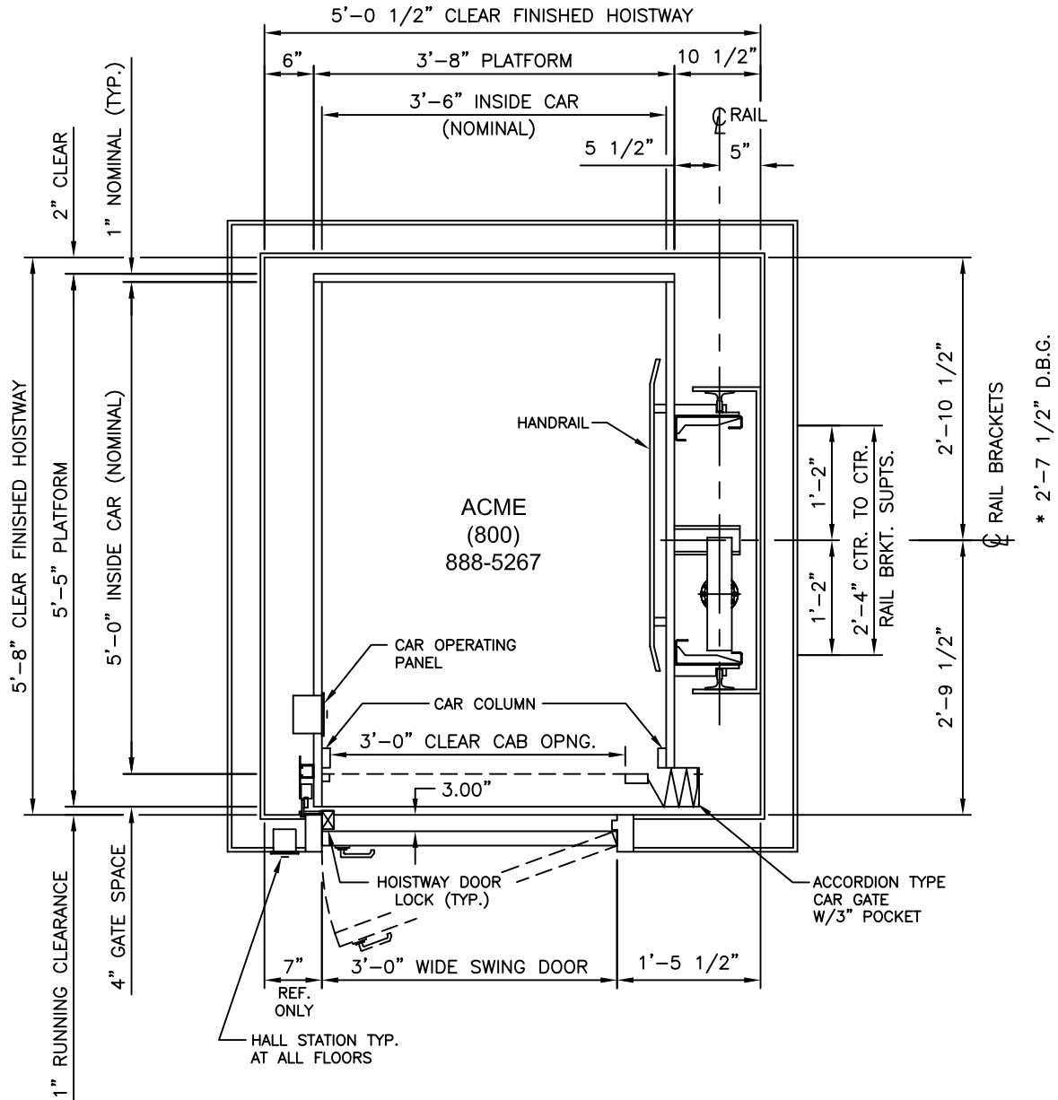
TYPICAL 1400-18 FLOOR PLAN SWING DOOR
